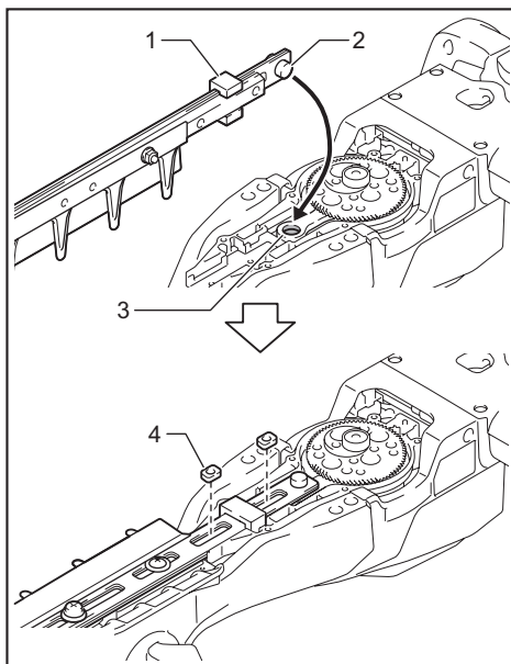
► 1. Felt pad 2. Protrusion 3. Hole 4. Sleeve
