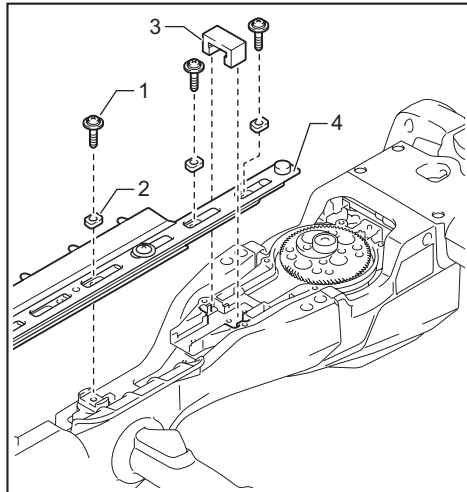
► 1. Screw 2. Sleeve 3. Felt pad 4. Shear blades
