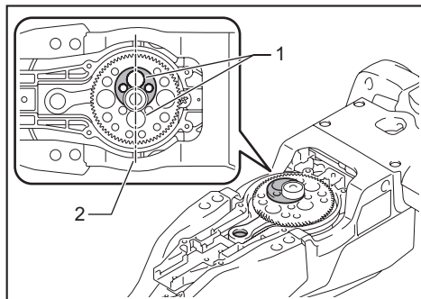
► 1. Hole 2. Alignment line
