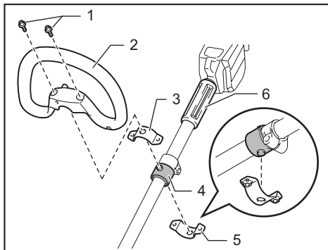
► 1. Hex socket head bolt 2. Handle 3. Upper clamp 4. Damper 5. Lower clamp 6. Spacer
