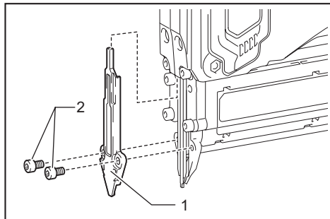
► 1. Driver guide cover 2. Hex bolt
