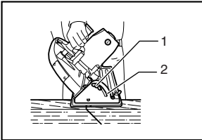
1. Clamping screw 2. Bevel scale plate
